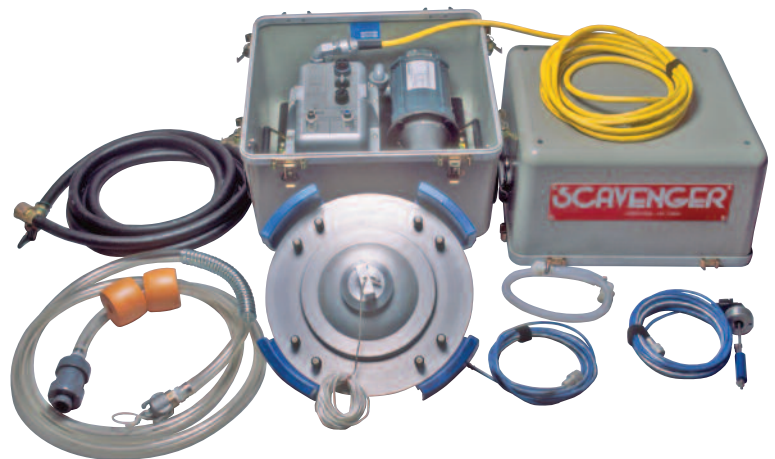
Large Diameter Filter Scavenger system with optional case
