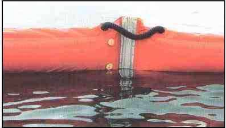
Oil Stop's single point inflation boom.
